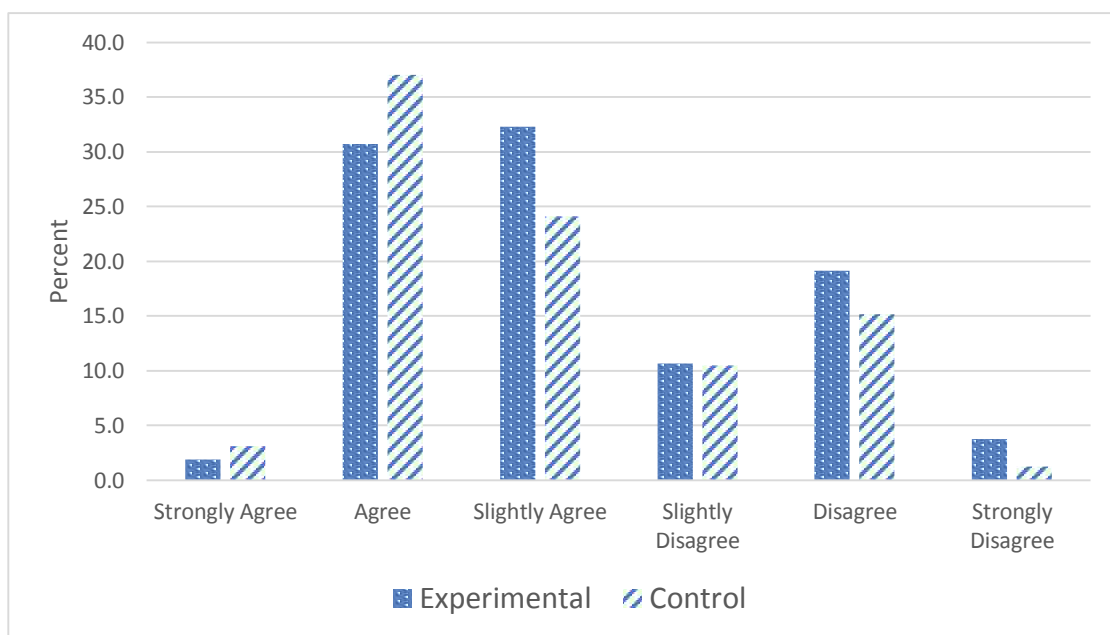
Figure 3. Responses to statement: The content of the exam was difficult.
