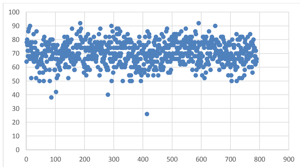
Figure 1. Scatterplot indicating outliers.
