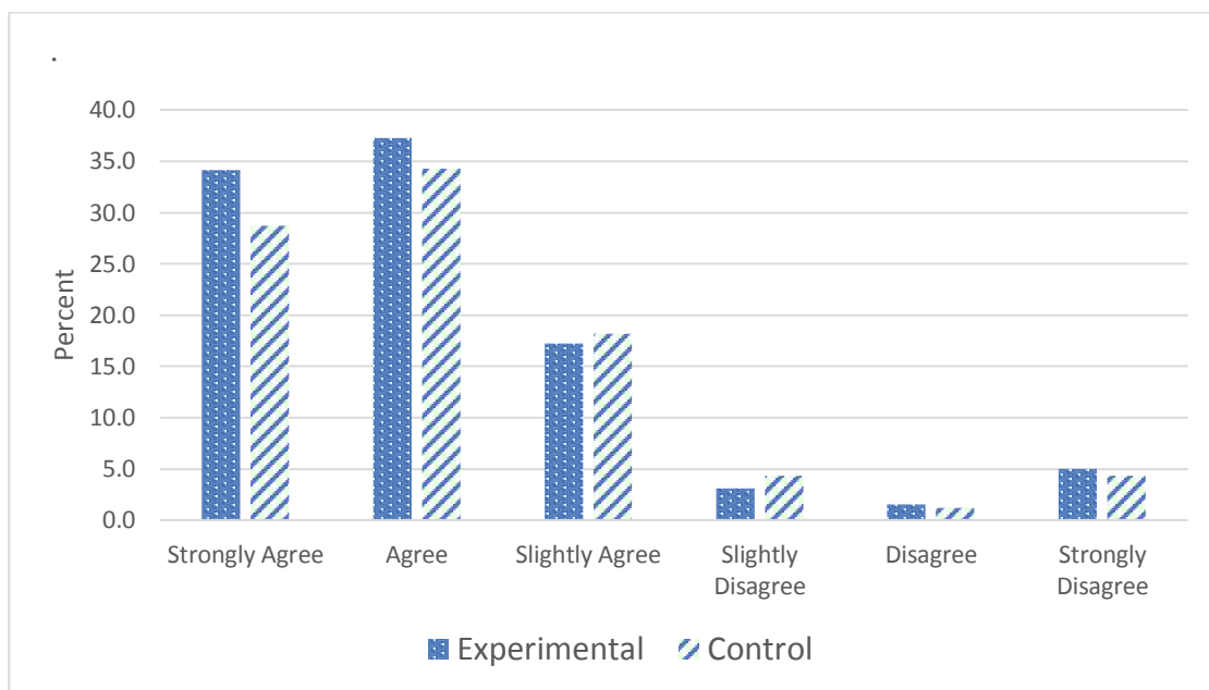
Figure 2. Responses to statement: Exam questions were clear and easy to understand.
